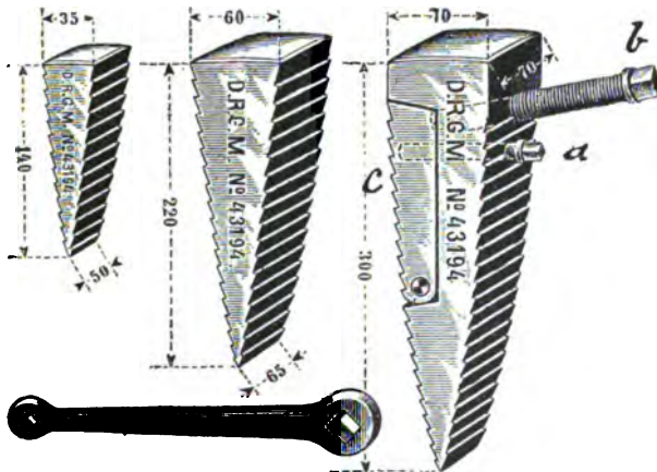
Fig. 123.—Schnücke's toothed wedge. Nos. are centimeters.
